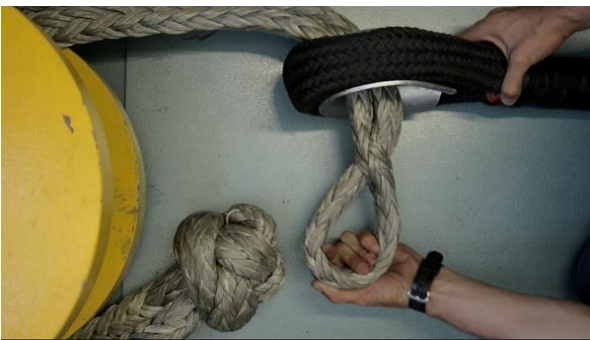
Step 4: Open soft shackle eye
