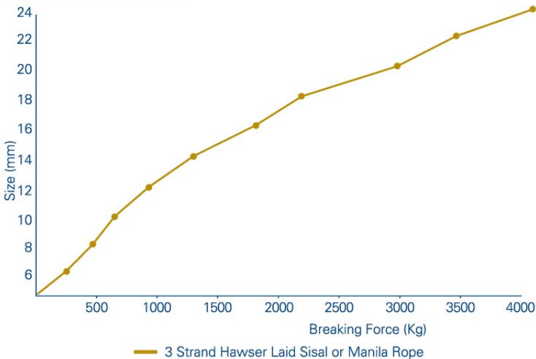
Breaking Force Graph
